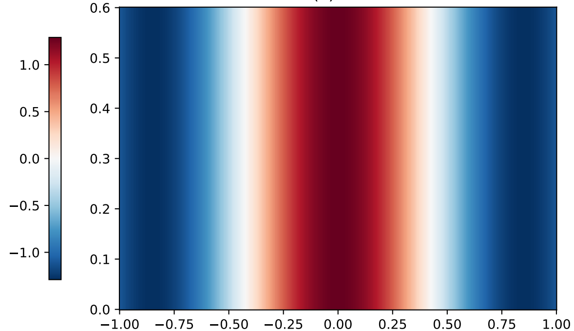
Re(u) Exact
